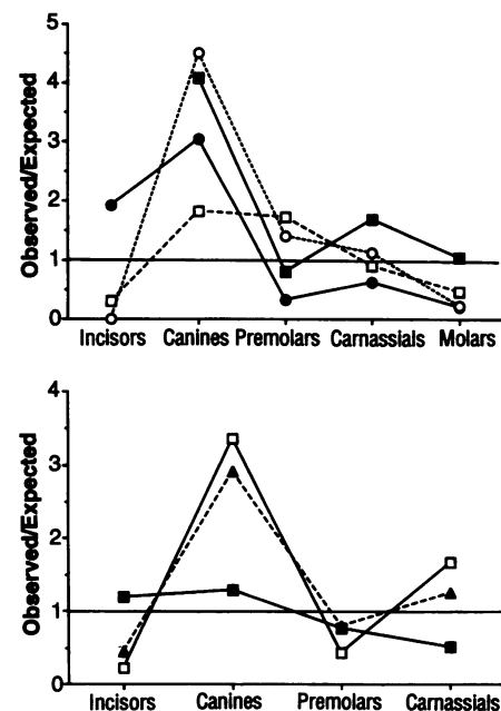
Fig. 1. The ratio of the observed over the expected number of broken teeth for each type of tooth within each species. Top: Canis dirus (●), Pleistocene C. latrans (RLB) (■), extant C. latrans (□), C. lupus (○). Bottom: Panthera leo (□), Panthera atrox (▲), Smilodon fatalis (■). For each species, the expected values were calculated as the product of the overall fracture frequency (Table 1) and the number of teeth represented in the sample for each position (Table 2). A value of 1 indicates the observed rate was equal to the expected rate. Tooth types as described in Table 2.
